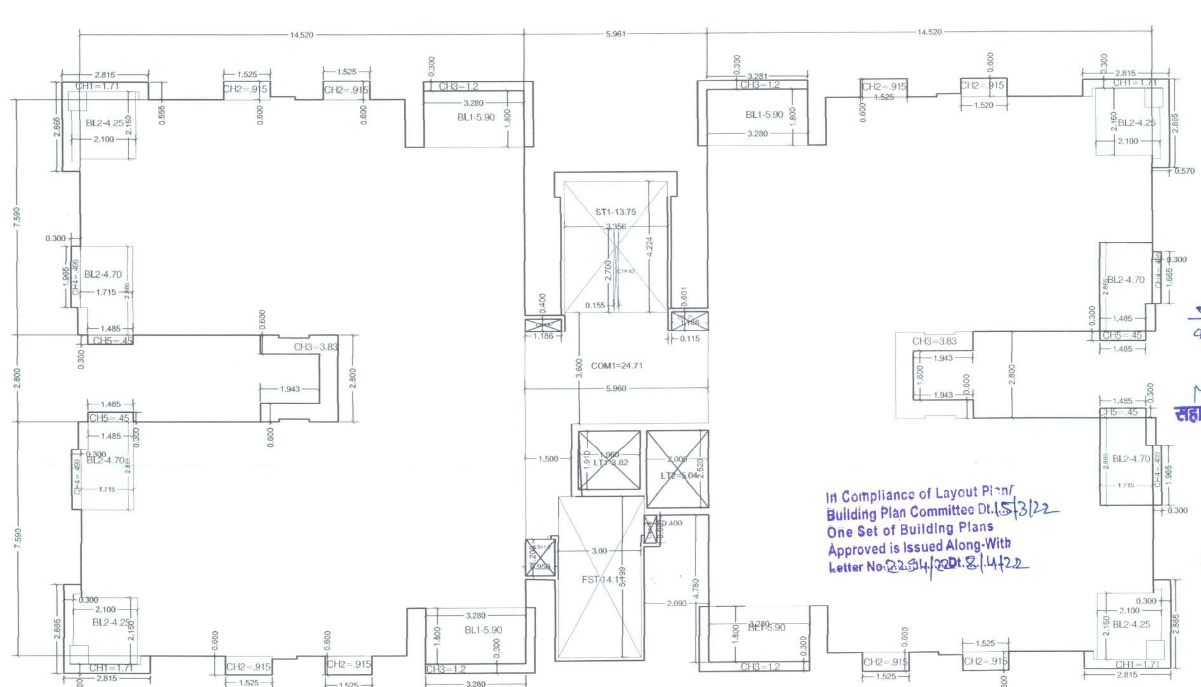
AREA DIAGRAM TYPICAL FLOOR
