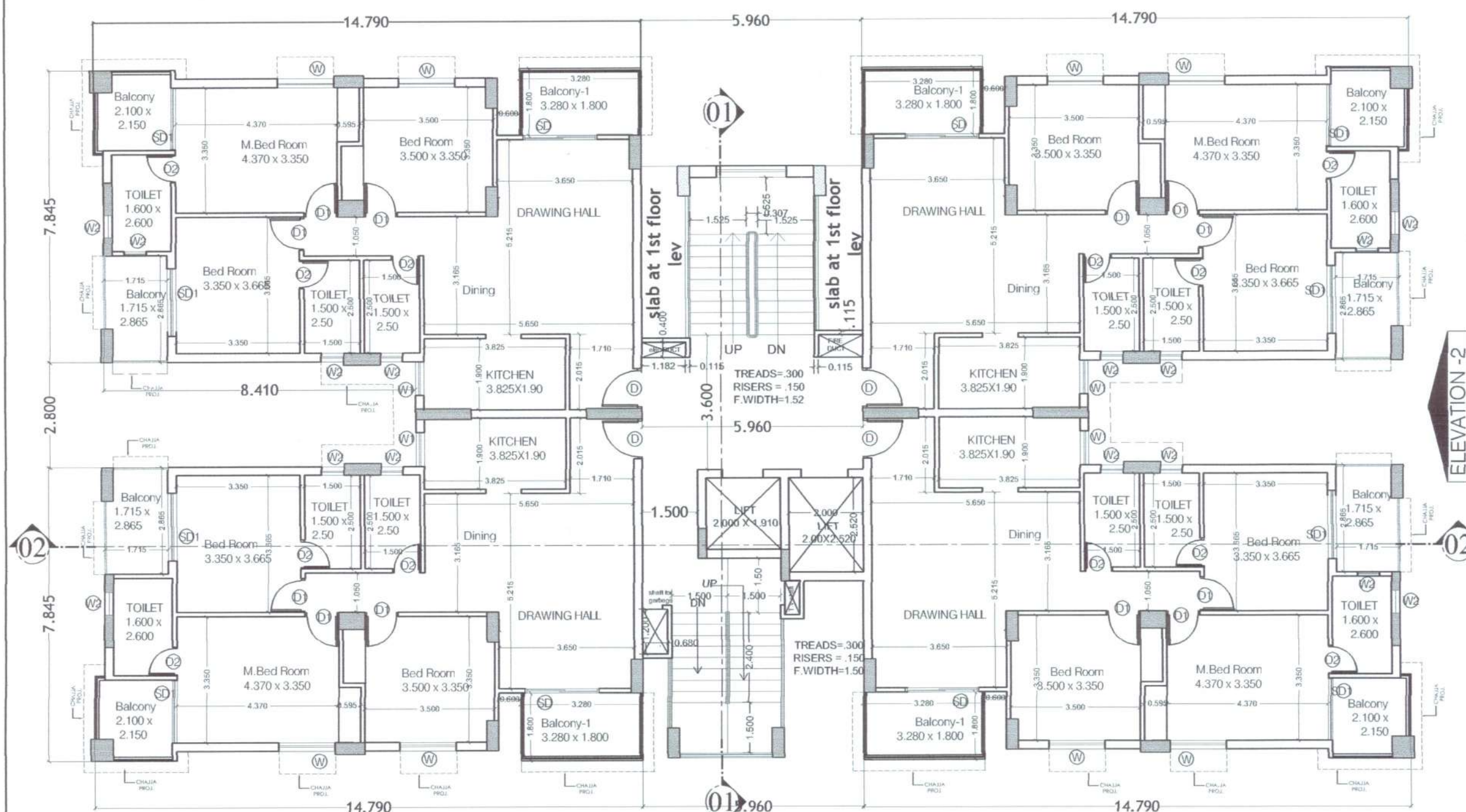
TYPICAL FLOOR PLAN 1ST TO 12TH FLOOR
