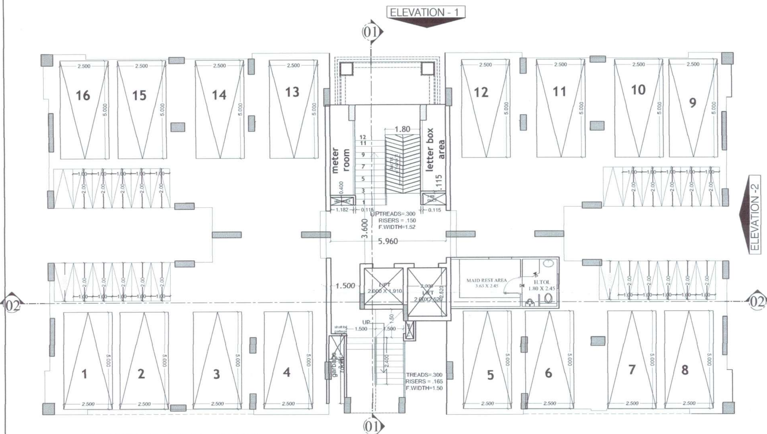
STILT FLOOR PLAN
